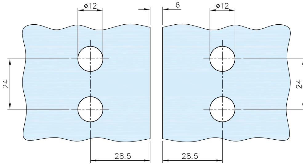
glass cutout
